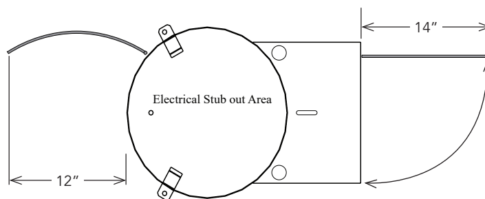
Recommended Clearance access for door openings
