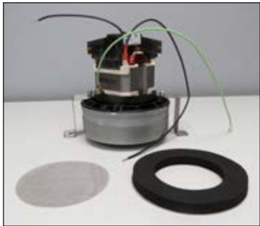
Part # 100041-00 Motor kit, 120v, contains 1 motor, 1 gasket and 1 screen
