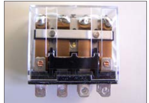
Part # 1902400 Relay, 4PDT
